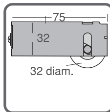
TT665 Single Loose Item Max. 50kg each COASTLINE SHEAVE CONCAVE WHEEL ALL STAINLESS STEEL
