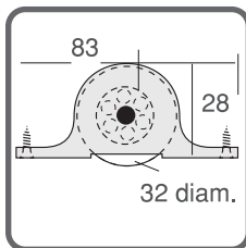
P661 Pack of 2 Max. 30kg each P671 Pack of 2 Max. 60kg each HORIZON SHEAVE 661 = NYLON WHEEL 671 = STEEL WHEEL
