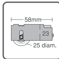
TT662 Single Loose Item Max. 20kg each JOINERY SHEAVE CONC. NYLON WHEEL #304 ST/STEEL CASING
