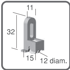
S978 Pack of 2 Max. 12kg each CONCAVE WHEEL SHEAVE FOR SLIDING WINDOW
