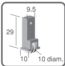
S980 Pack of 2 Max. 12kg each CONCAVE WHEEL SHEAVE FOR SLIDING WINDOW
