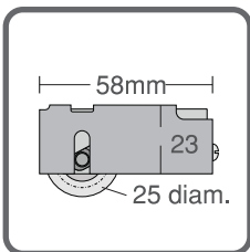
TT663 Single Loose Item Max. 30kg each JOINERY SHEAVE CONCAVE WHEEL ALL #304 ST/STEEL
