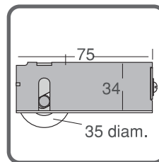
TT657 Single Loose Item Max. 100kg each TIMBERLINE SHEAVE WITH CONCAVE BRONZE WHEEL
