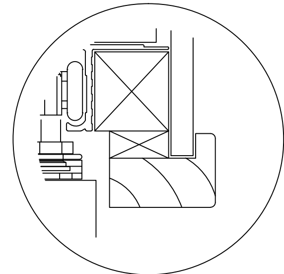
30mm REBATED JAMB OPTION.
