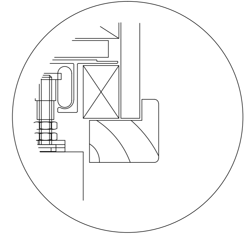
30mm REBATED JAMB OPTION.
